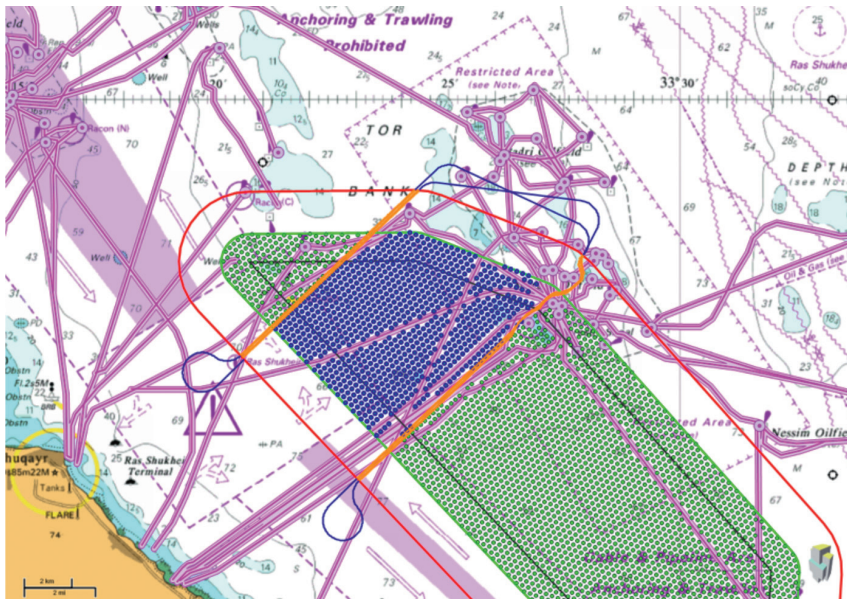
Figure 5 OBN design around obstructed area and shipping lanes, showing 200 x 200m receivers, with H pattern roll. Shots for the current patch are shown in orange, with active receivers in blue.
